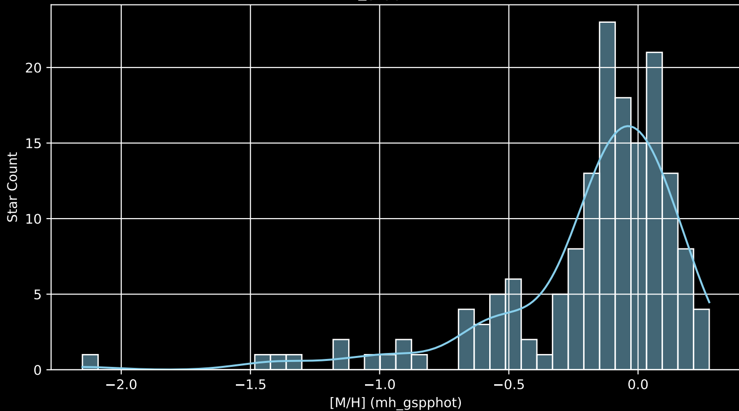
APOGEE DR17 Field: [090+12 [M/H] (mh_gspphot) (n= 160)
