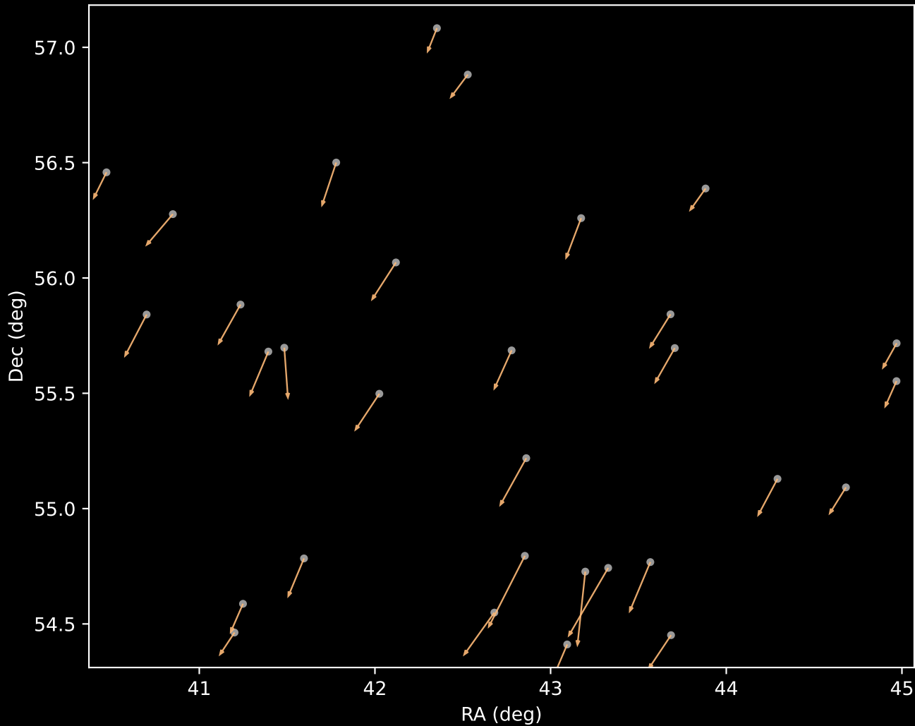
APOGEE DR17 Cluster 3 Proper Motion Vectors (n=31)
