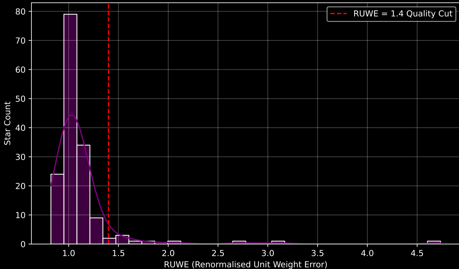
GAPOGEE DR17 Field [090+12] RUWE Distribution (n= 157)
