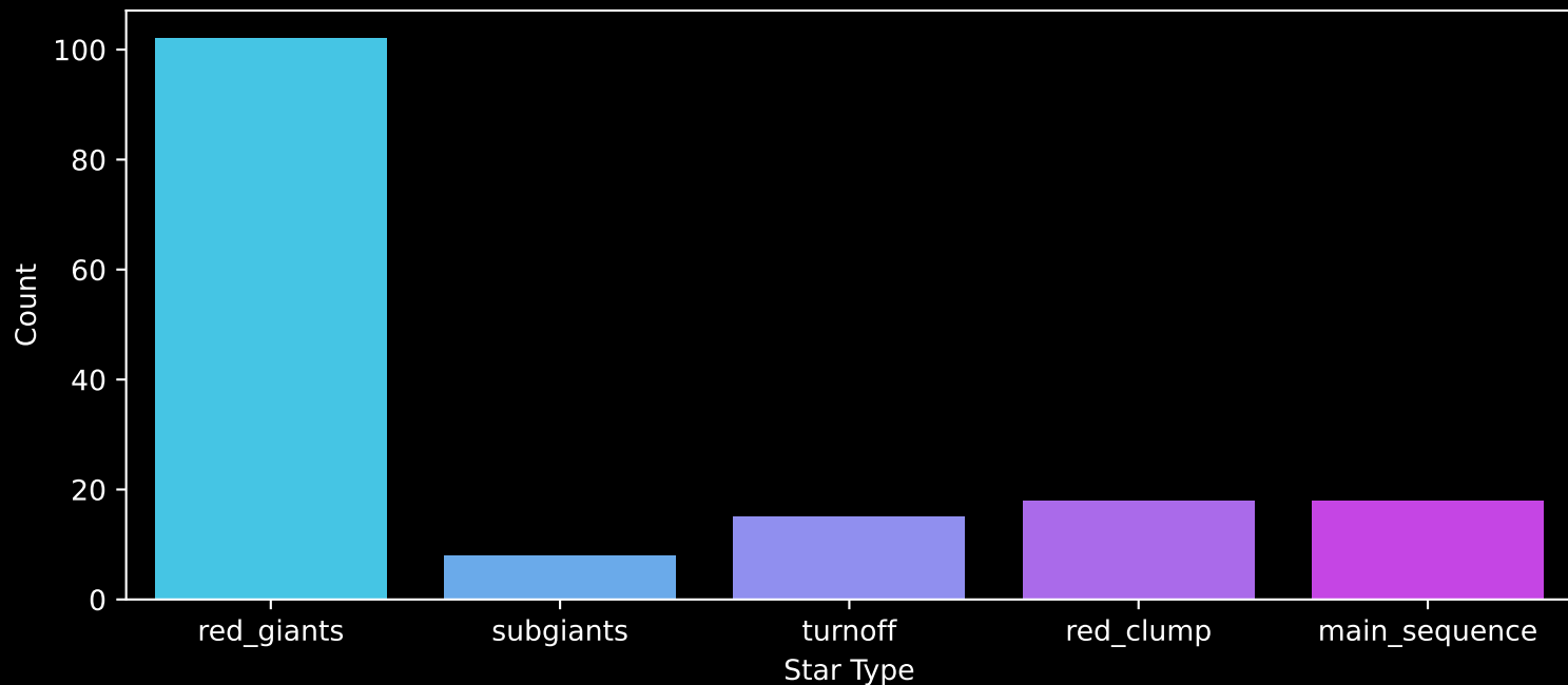
APOGEE DR17 Field: [090+12] Count plot of Star Type
