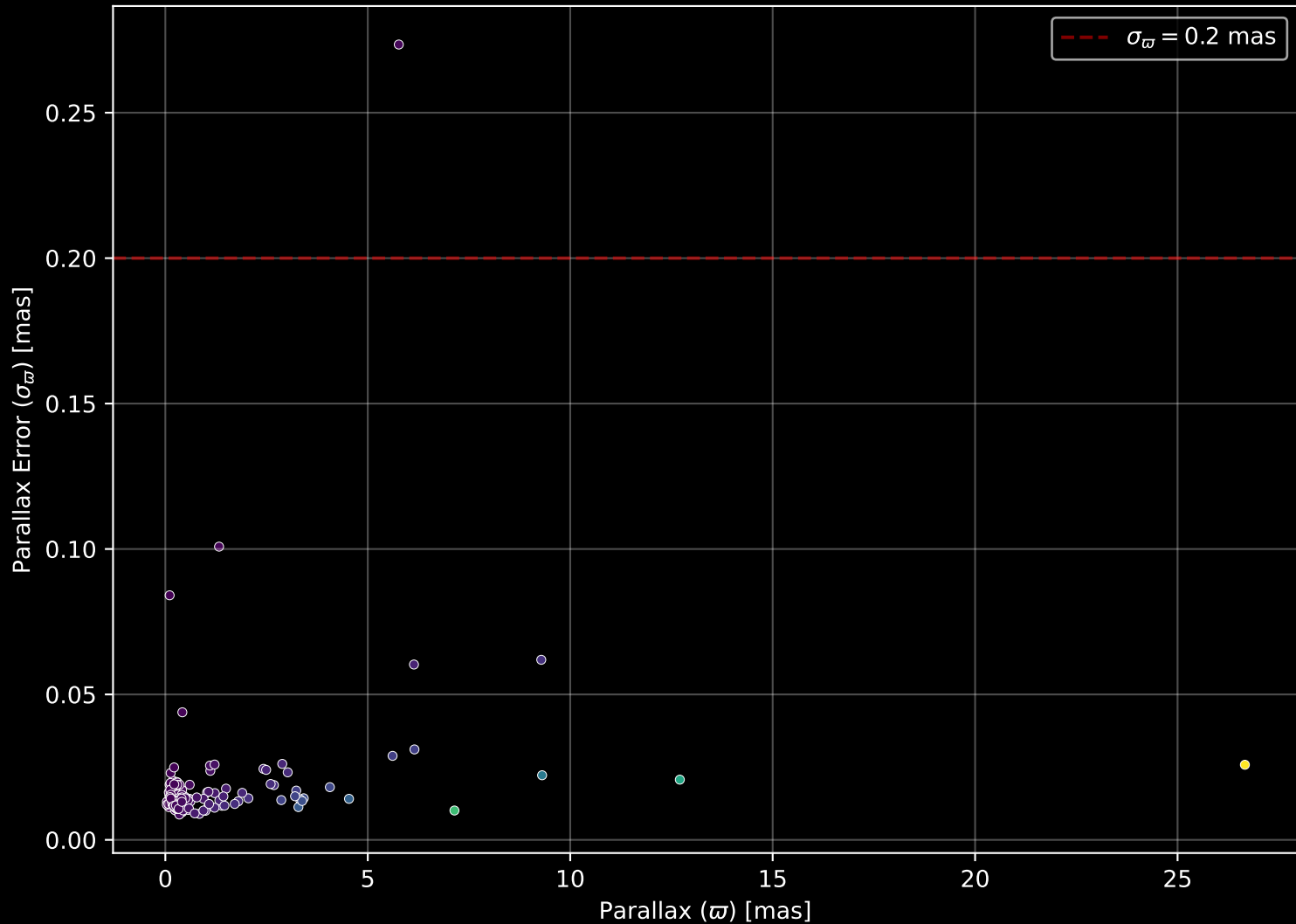
APOGEE DR17 Field: [090+12] Parallax Quality (n= 161)
