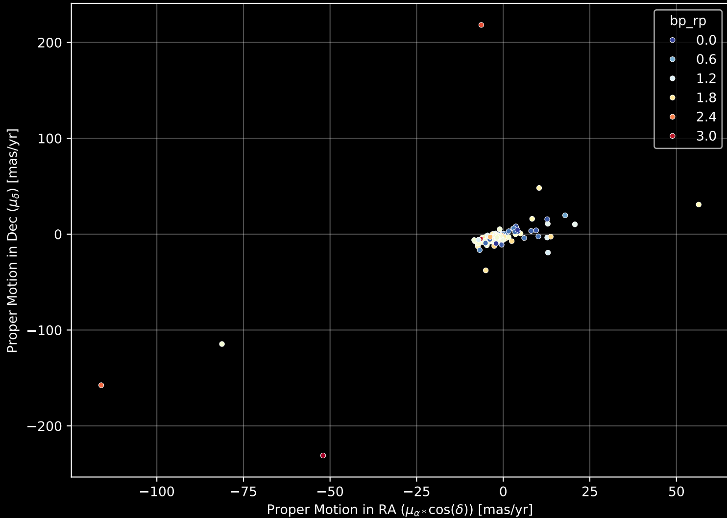
APOGEE DR17 Field: [090+12] Proper Motion Diagram (n= 161)
