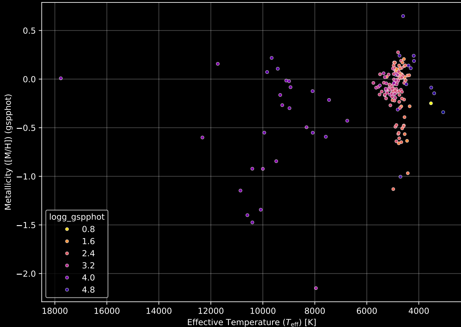
APOGEE DR17 Field: [090+12] Stellar Population Parameters (n= 161)
